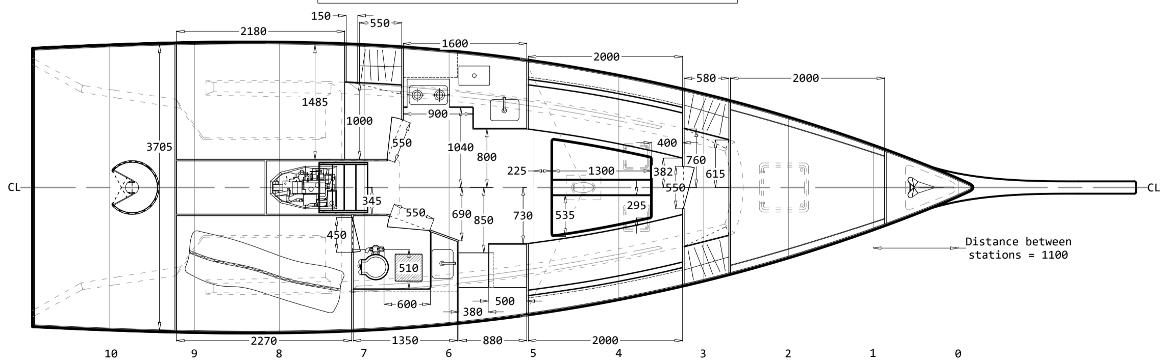
View of interiors - Top view
