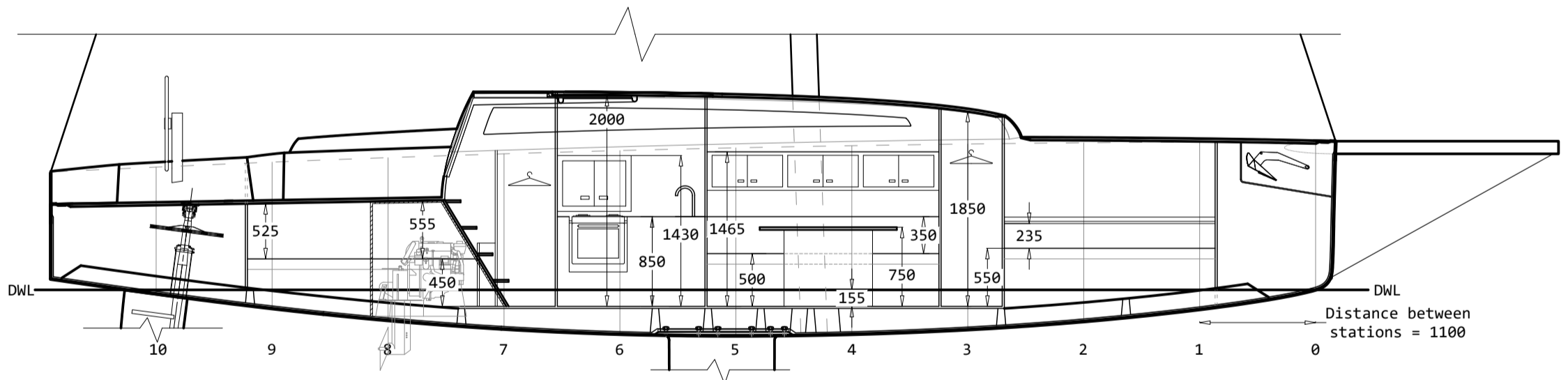
View of interiors - Centerline to port
