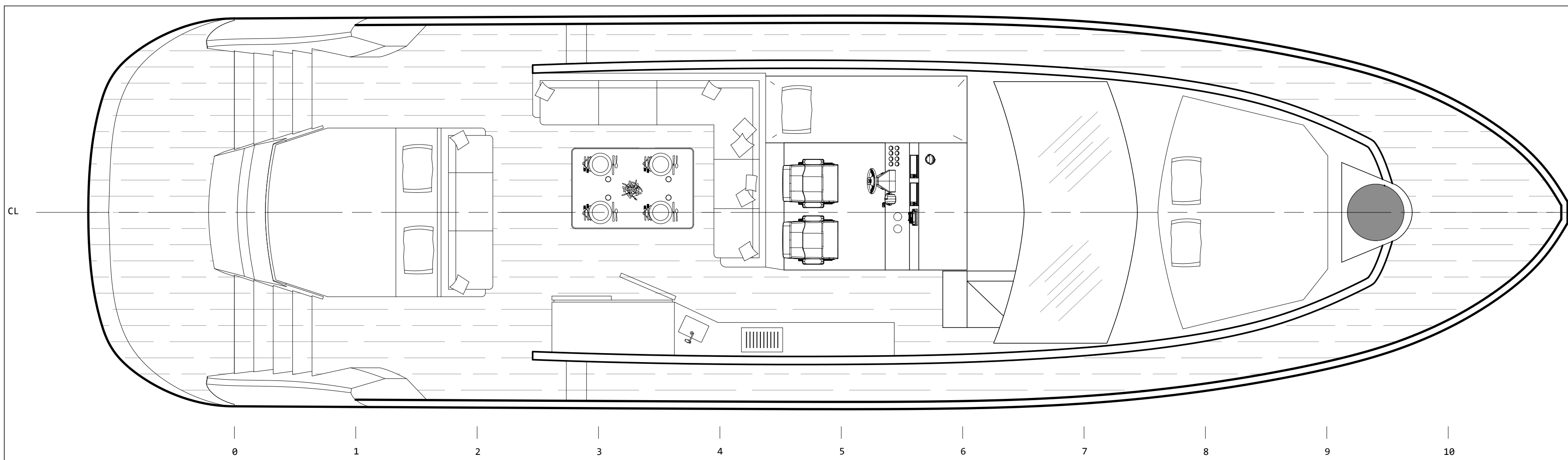
Piso 1: General
